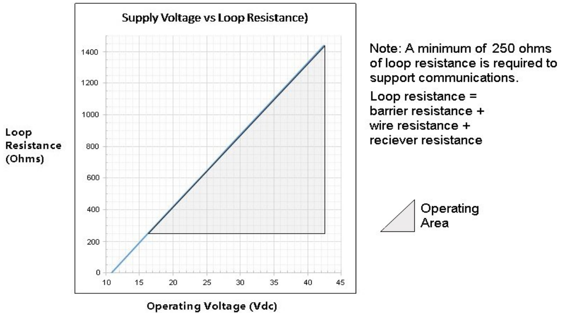
2 - Supply voltage and loop resistance chart & calculations
