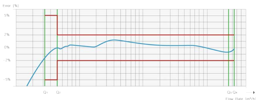
BECO X Ultrasonic Water Meter Accuracy Curve
