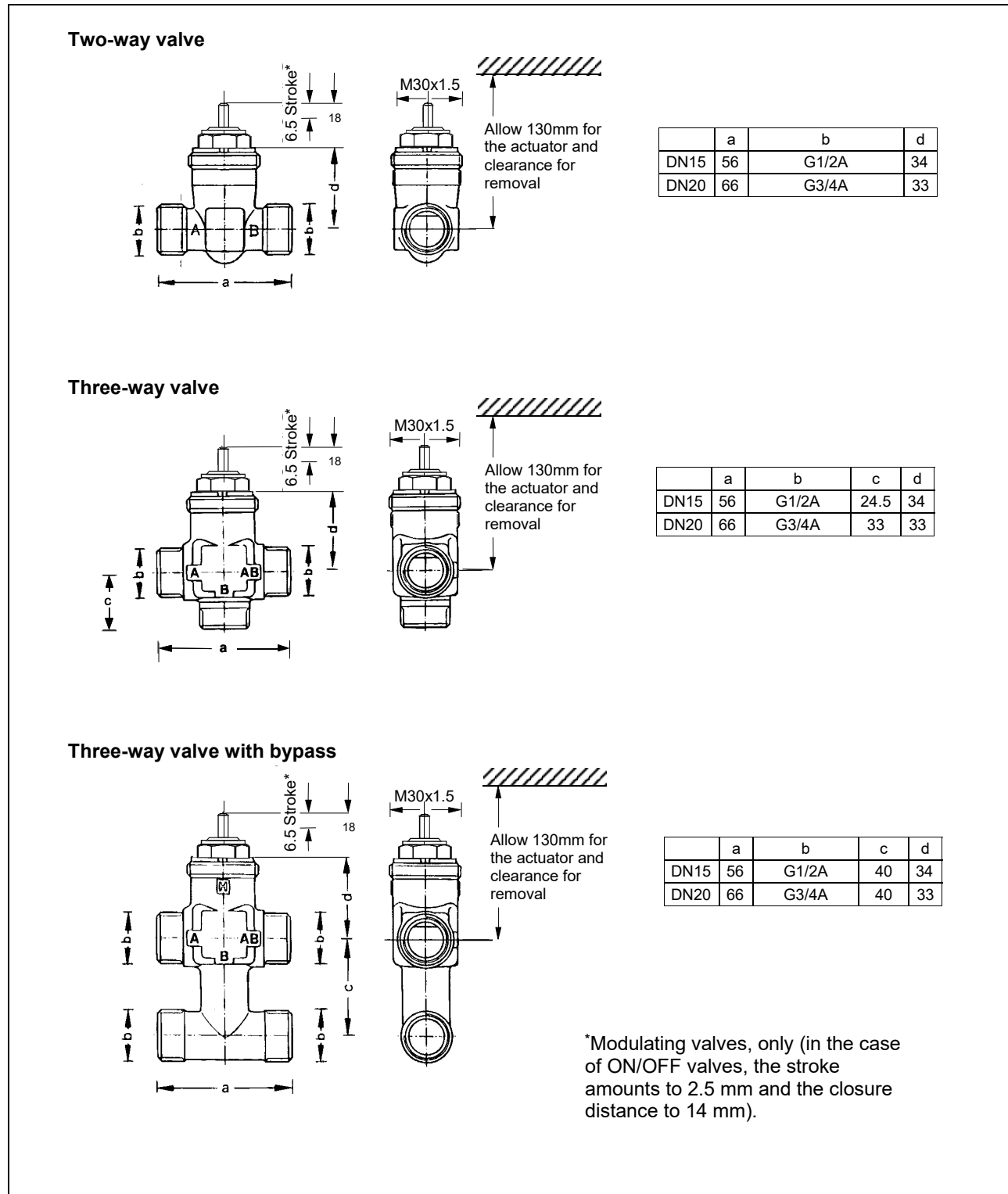
Fig. 4. Dimensions V5832A/V5833A,C in mm
